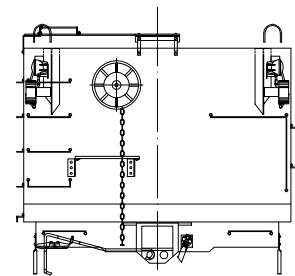
End View West (leftside)
