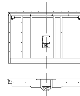
End View East (rightside)
